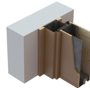
E – Corridor frame in block.
