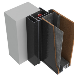
D – Metal pre-frame with plate finished with metal cover.
